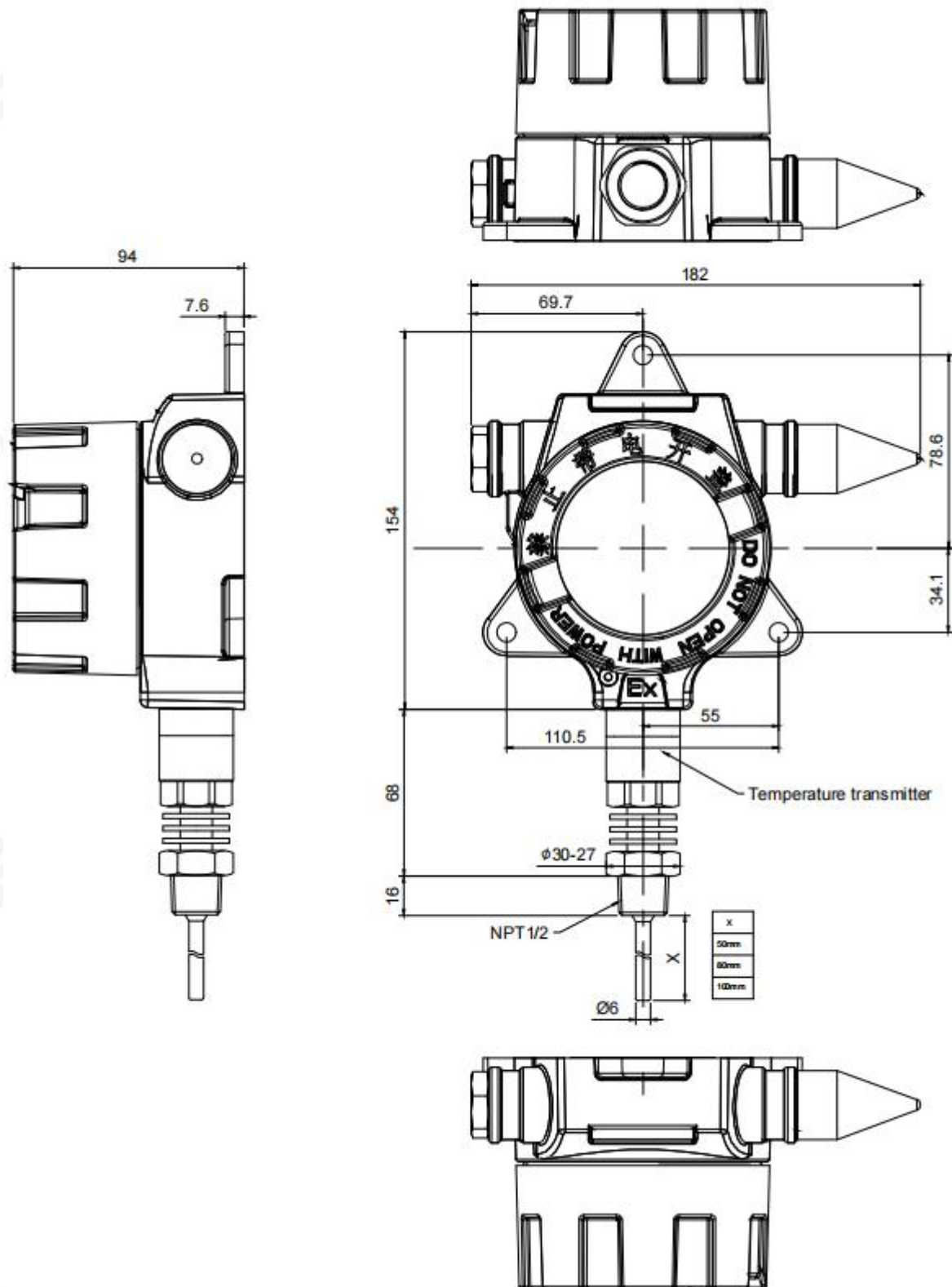
Temperature sensor, model No. MZW2602
