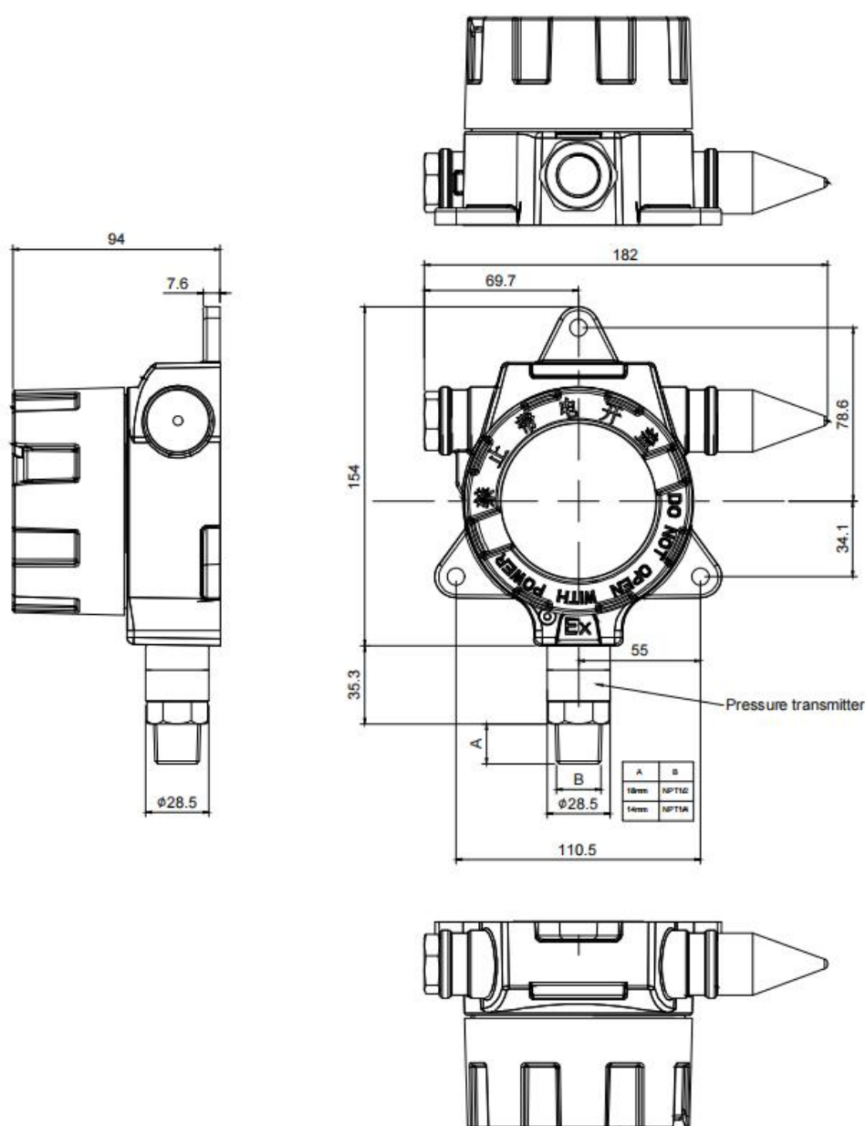
Pressure sensor, model No. MZW2601
